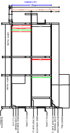
SECTION "A-B"
