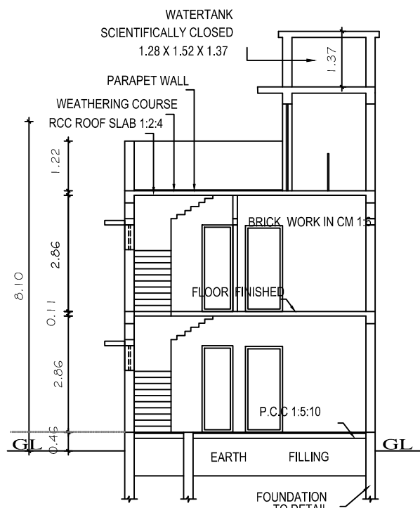
SECTION "A-B"
