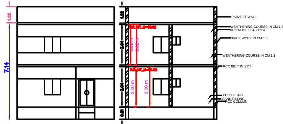
ELEVATION SECTIONON-"AA"&"BB"
