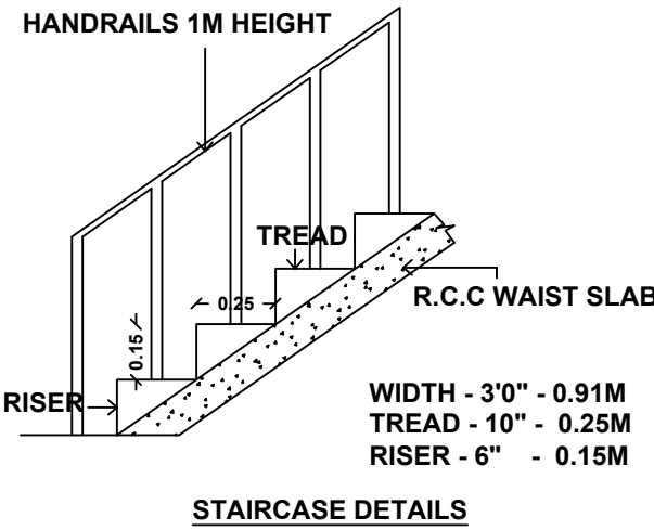
STAIRCASE DETAILS
