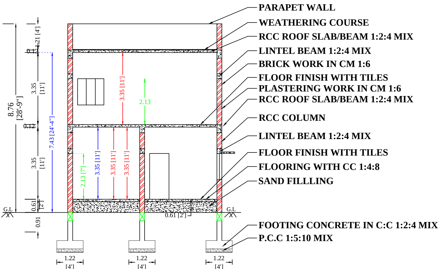
SECTION - "AA"
