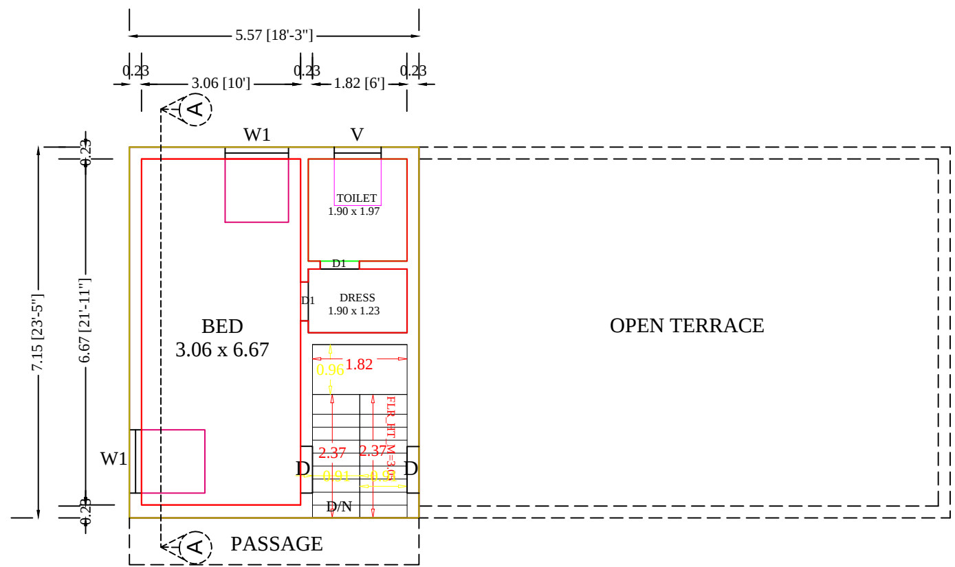
PRO.FIRST FLOOR PLAN
