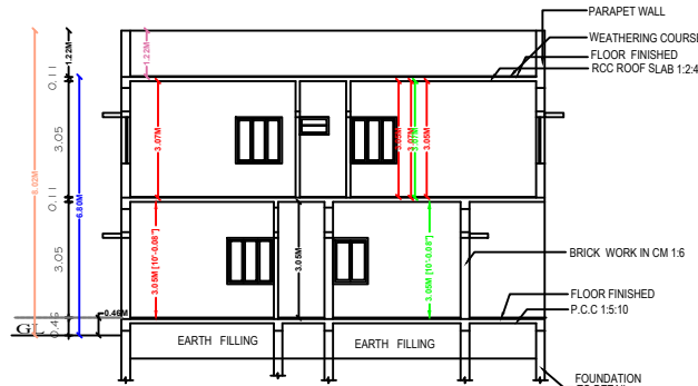
SECTION "A-B"
