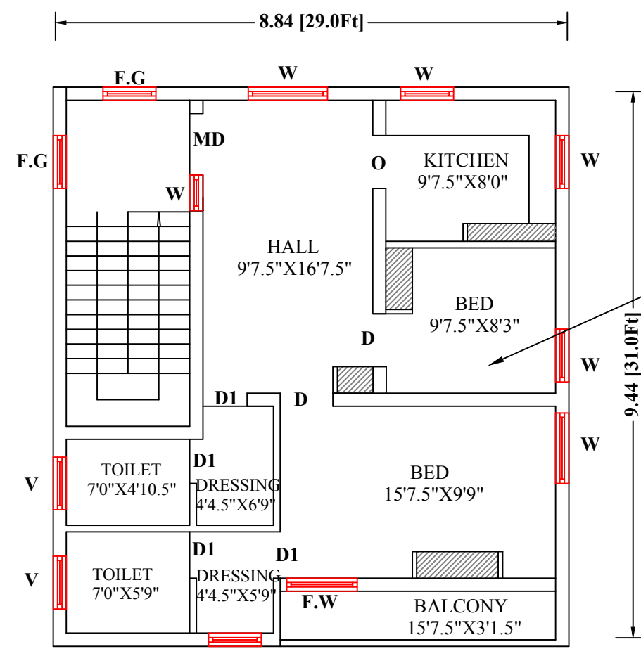
FIRST FLOOR PLAN -RESIDENTIAL
