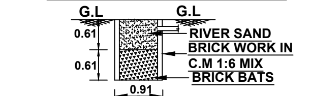
. SECTION ON RAIN WATER COLLECTION TUB .
