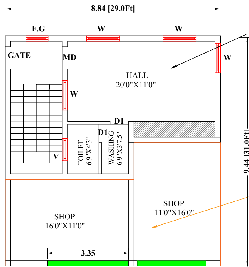
GROUND FLOOR PLAN- COMMERCIAL & RESIDENTIAL
