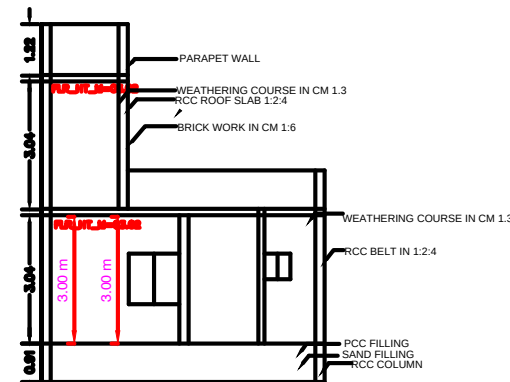
SECTIONON-"AA"&"BB"
