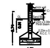
FOUNDATION DETAIL
