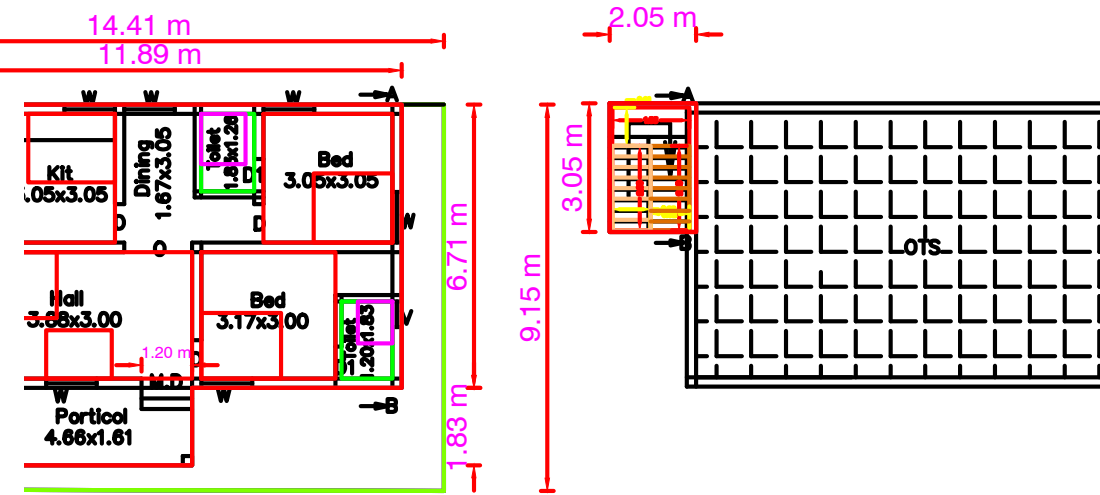
FIRST FLOOR(Pro.)
