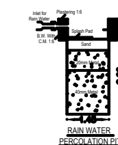
RAIN WATER PERCOLATION PI
