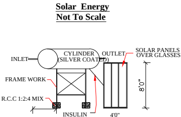
Waste Water Recycle Unit Not To Scale
