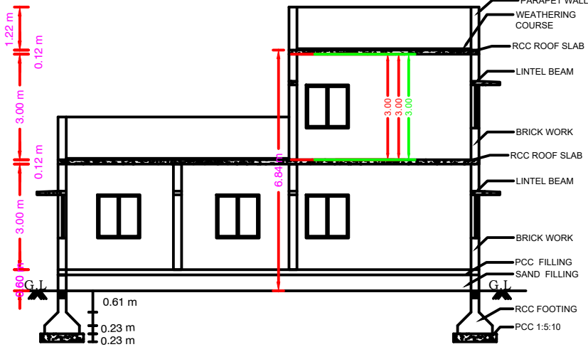
SECTION ON KA
