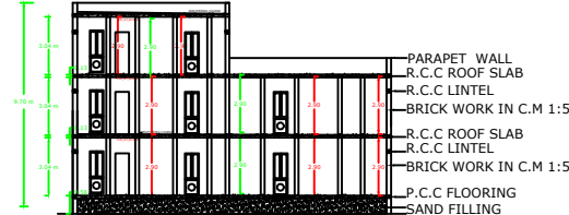
SECTION ON K-S
