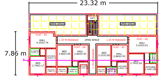
PROPOSED SECOND FLOOR PLAN
