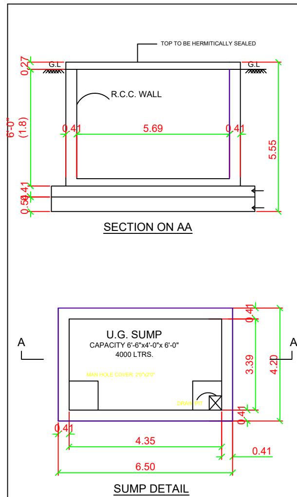
SUMP DETAIL
