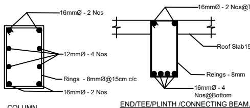
COLUMN
