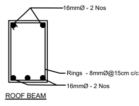
ROOF BEAM
