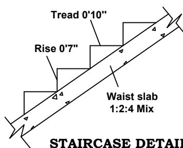
STAIRCASE DETAILS (NOT TO SCALE)
