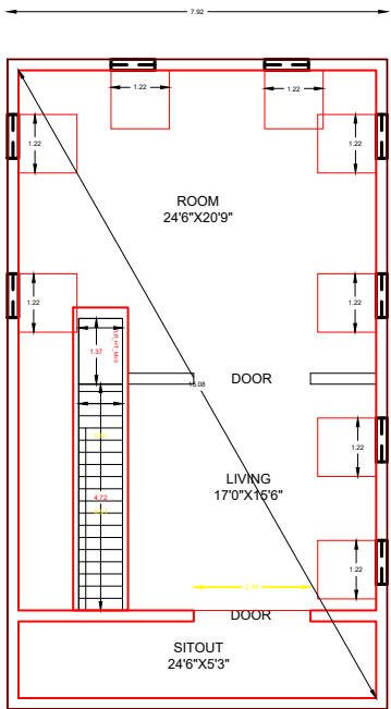
GROUND FLOOR PLAN [WEST FACING]
