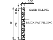
DETAILS OF PERCOLATION PIT
