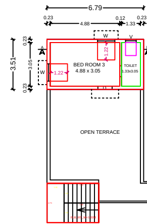
PROPOSED FIRST FLOOR PLAN (EAST FACING)
