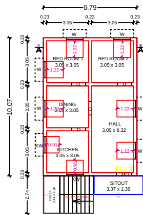
EXISTING GROUND FLOOR PLAN (EAST FACING)
