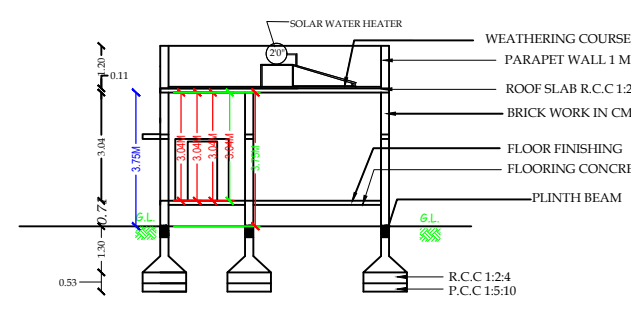
"A-A" SECTION
