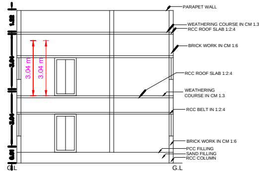
SECTION ON-AA&BB
