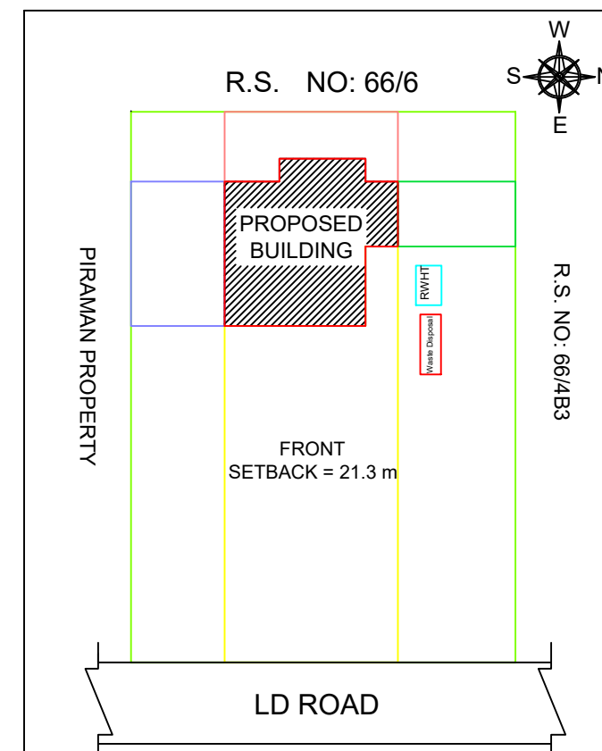
SITE PLAN
