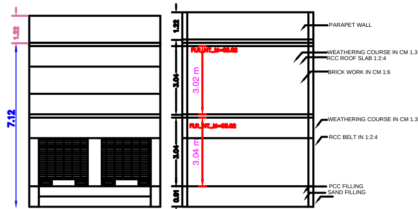
ELEVATION SECTIONON-"AA"&"BB"
