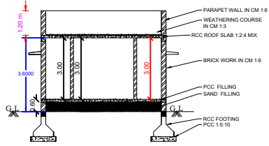
SECTION-"SR"
