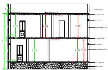
SECTION ON K-S
