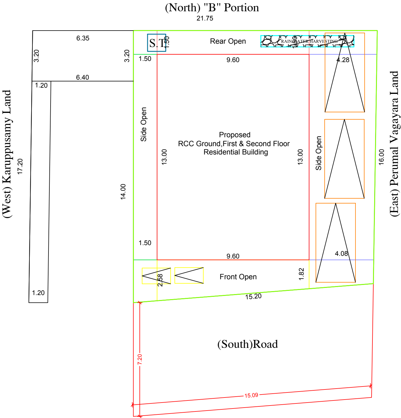
TOPO PLAN SITE REFERENCE
