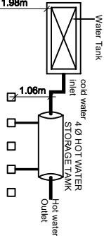
SOLAR HOT WATER SYSTEM (SWHS) DETAIL
