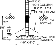
FOUNDATION DETAIL
