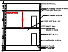
SECTION ON-AA&BB
