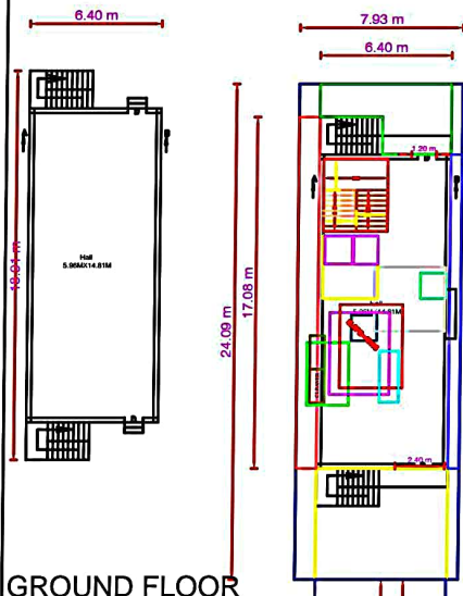
GROUND FLOOR (CO)
