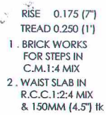
STAIRCASE SECTION
