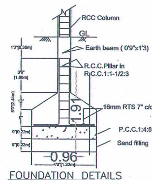
FOUNDATION DETAILS
