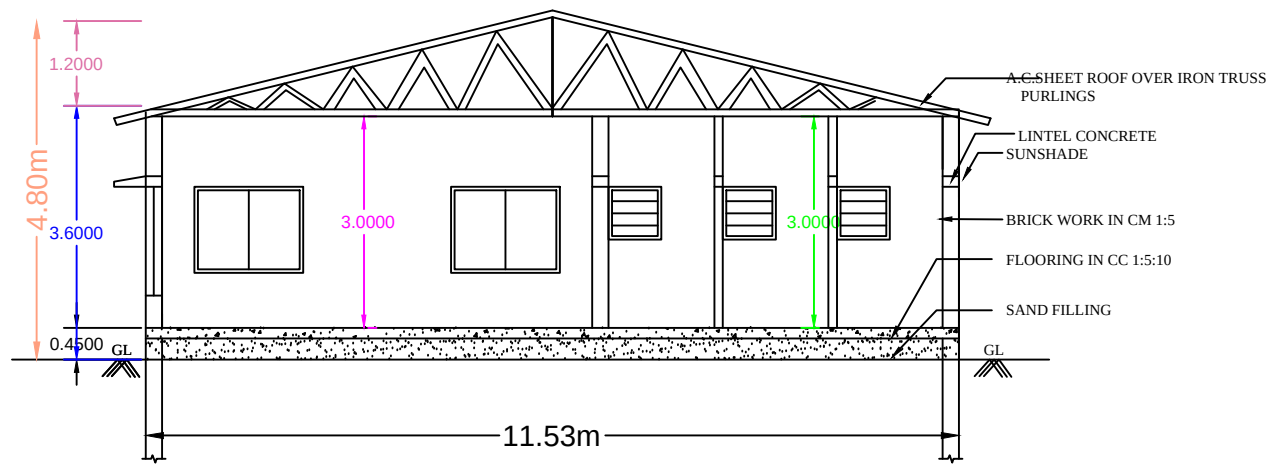
SECTION AB
