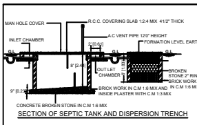
SECTION OF SEPTIC TANK AND DISPERSION TRENCH
