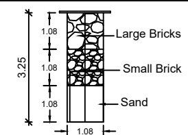
SECTION OF RAIN WATER COLLECTION PITS (NTS)
