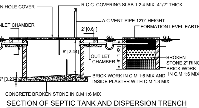
SECTION OF SEPTIC TANK AND DISPERSION TRENCH
