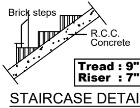
STAIRCASE DETAILS
