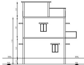
FRONT ELEVATION
