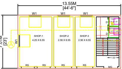
PROPOSED GROUND FLOOR PLAN EAST FACING
