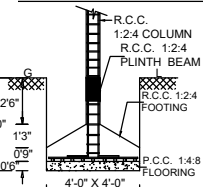
FOUNDATION DETAIL
