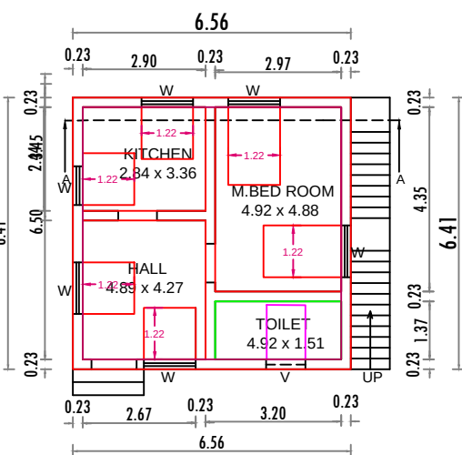
FLOOR - GROUND
