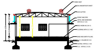
SECTION ON "AB"
