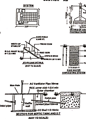
SECTION "AB"
