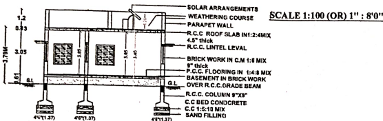
SECTION "AB"
