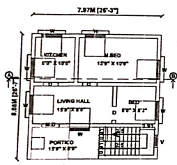
GROUND FLOOR PLAN ( NORTH FACING )
