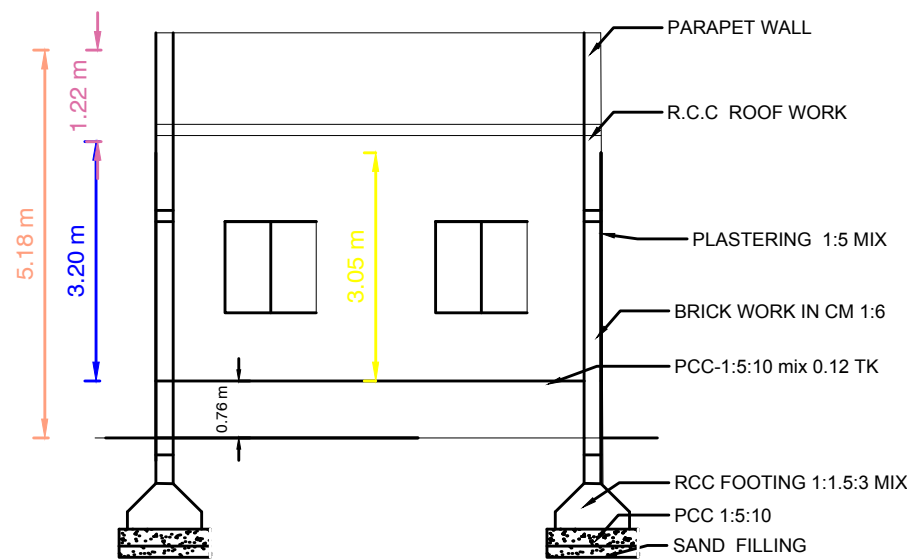
SECTION"AB"
