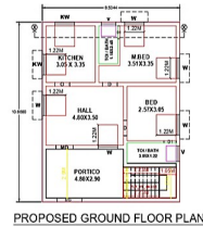
PROPOSED GROUND FLOOR PLAN
