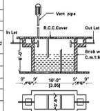
SEPTIC TANK DETAILS (NOT TO SCALE)
