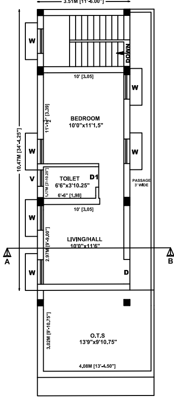
PROPOSED SECOND FLOOR PLAN
