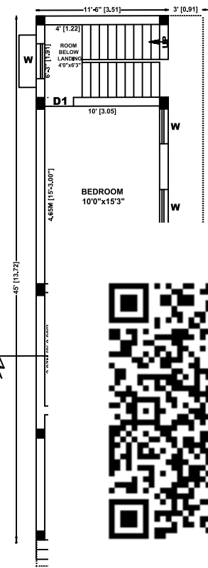
EXISTING GROUND FLOOR PLAN
