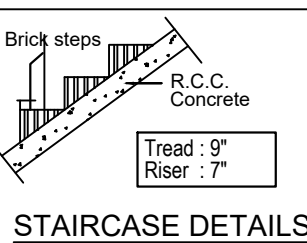
STAIRCASE DETAILS
