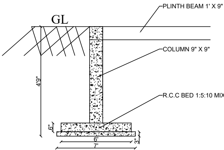
FOOTING DETAILS
