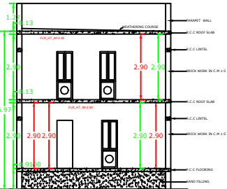
SECTION ON K-S
