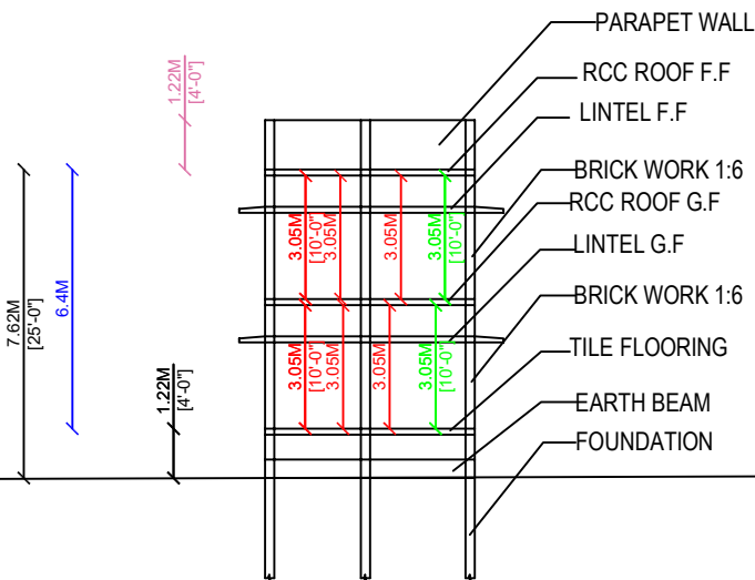
SECTION "A-B"
