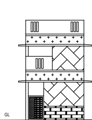
FRONT ELEVATION.
