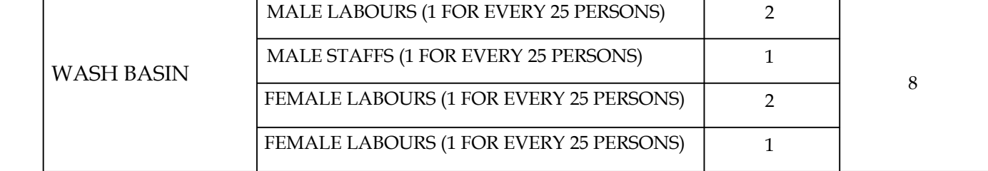
BLOCK - 11 (Toilet) (Ground Floor Plan) (Fully Mechanical Ventilation)
