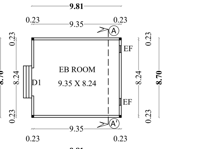
BLOCK - 2 (EB ROOM) (Ground Floor Plan) (Fully Mechanical Ventilation)
