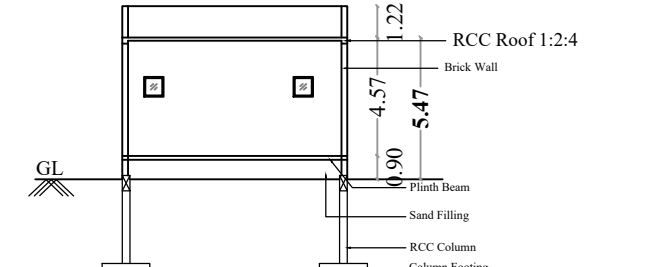
BLOCK - 2 (Section A-A')
