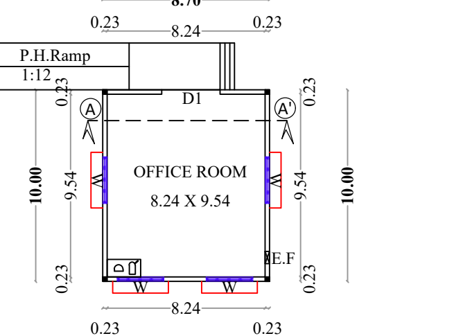
BLOCK - 3 (OFFICE ROOM) (Ground Floor Plan) (Fully Mechanical Ventilation)
