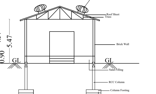
BLOCK - 3 (Section A-A')
