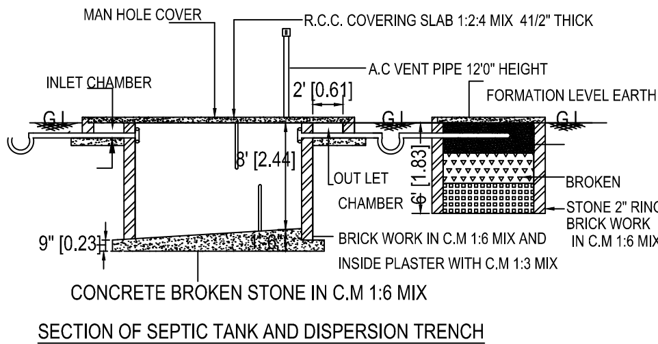
SECTION OF SEPTIC TANK AND DISPERSION TRENCH
