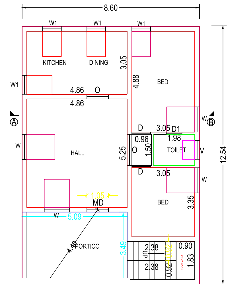
FLOOR PLAN
