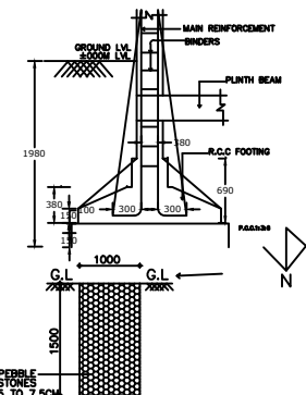
SECTION OF PEBBLE TRENCH
