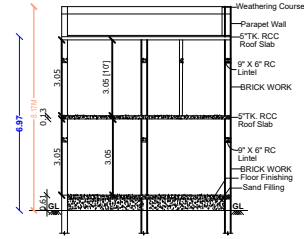
SECTION ON "SR"
