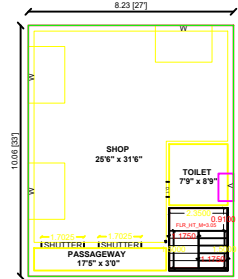
PROPOSED FIRST FLOOR
