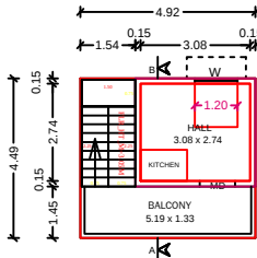
FIRST FLOOR PLAN (NORTH FACING)
