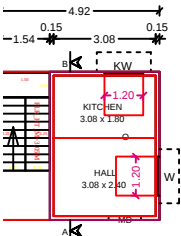
GROUND FLOOR PLAN (NORTH FACING)
