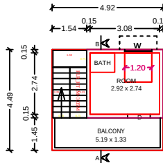
SECOND FLOOR PLAN (NORTH FACING)
