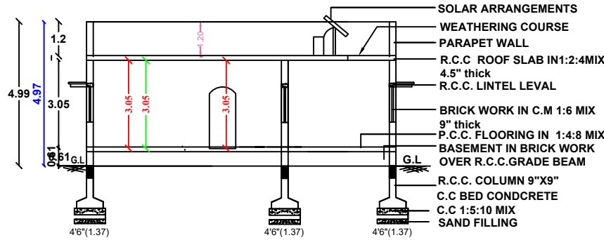
SECTION " AB "
